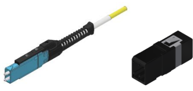
MDC Connector
